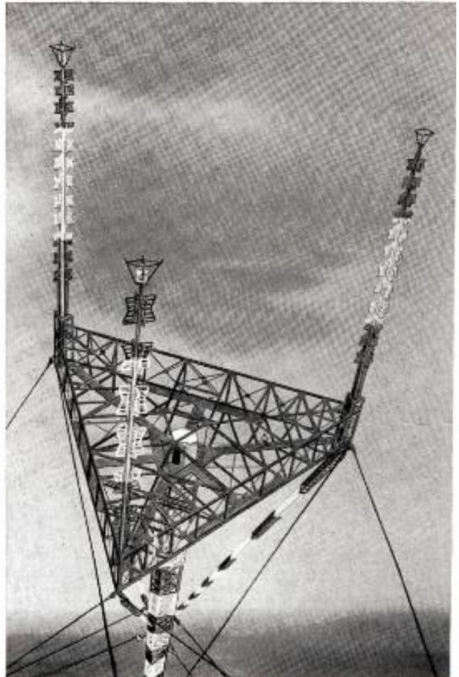
In the design above, three antennas occupy all of the corners, thus spreading the cost of the complete installation over three stations.
